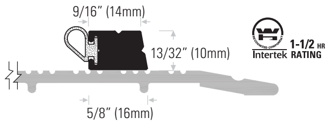
DST17BL Replacement TPE (T) insert black, for DS176N
