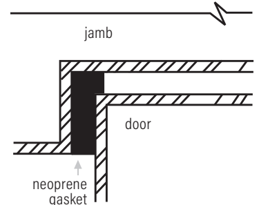
OVERHEAD VIEW
