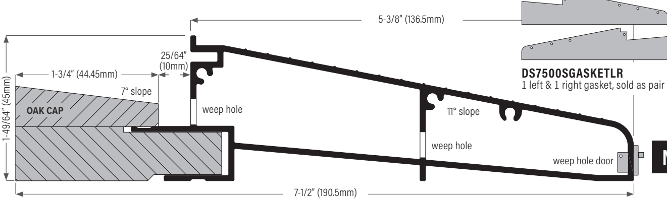
DS7500COAK Clear anodized with oak cap DS7500DOAK Bronze anodized with oak cap
