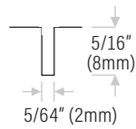
Required kerf slot size for DS435
