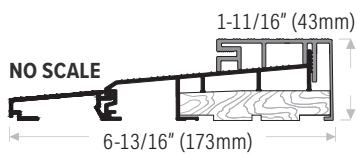
DS457 Sill shown with DS1122, 2" (51mm) extension
