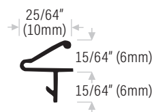
DSPF109T Extruded PVC/tan. Length available: 12ft (3658mm) only.
