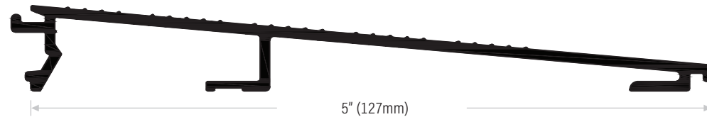
DS1115A150 Extruded aluminum mill finish. Length available: 150" (3810mm) only
