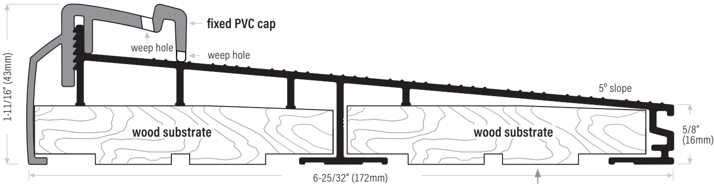
DS228W PVC white. 36", 48"
