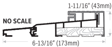
DS457 Sill shown with DS1122, 2" (51mm) extension
