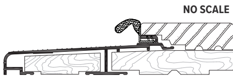
DS421 Used in outswing door sill application
