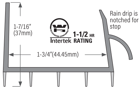
DS128BL PVC black. 36" only DS128B PVC brown. 36", 48" DS128W PVC white. 31-3/4", 32", 35-3/4", 36", 48"
