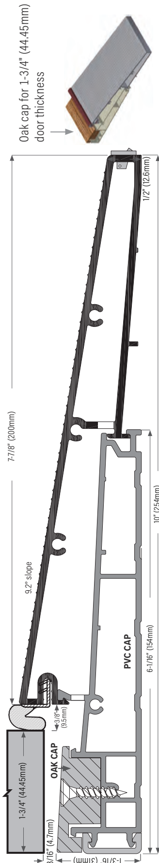
DS1051AOAK Mill finish with oak cap DS1051DOAK Bronze anodized with oak cap
