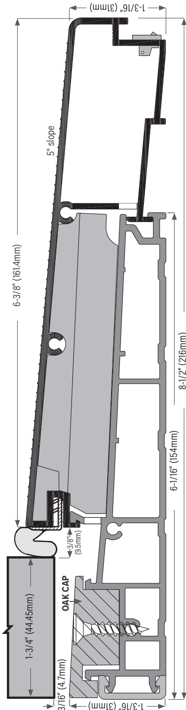
DS850AOAK Mill finish with oak cap DS850DOAK Bronze anodized with oak cap
