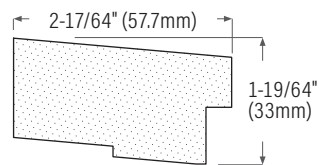
DS850SILLPLUG For DS850 & DS852 sills
