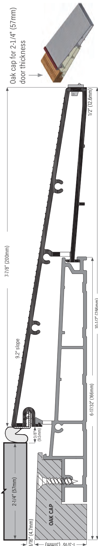
DS1052AOAK Mill finish with oak cap for 2-1/4" (57mm) door DS1052DOAK Bronze anodized with oak cap for 2-1/4" (57mm) door
