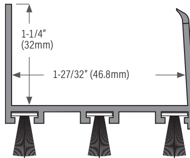
DS125B PVC brown. Lengths available: 36" only DS125W PVC white. 36", 48"
