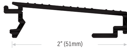
DS1122A150 Extruded aluminum mill finish. Length available: 150" (3810mm) only
