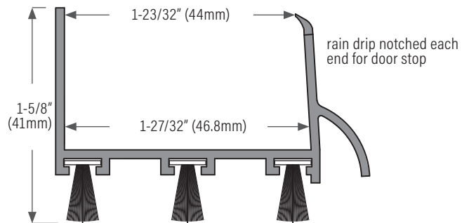
DS124BL PVC black. 36", 48" DS124B PVC brown. 36", 48" DS124W PVC white. 31-3/4", 32", 35-3/4", 36", 48"
