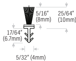
DSP108-35BL 5/16" (8mm) pile height, black
