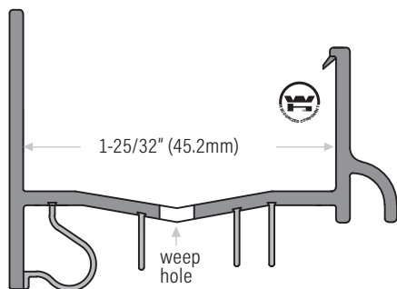
DS228W PVC white. 36", 48"
