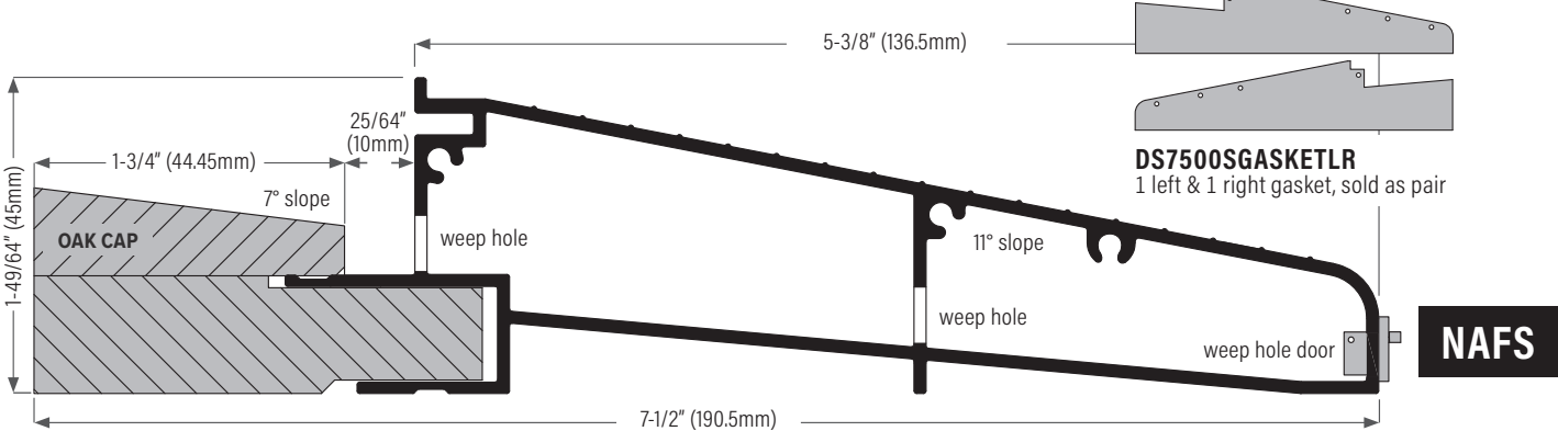
DS7500COAK Clear anodized with oak cap DS7500DOAK Bronze anodized with oak cap
