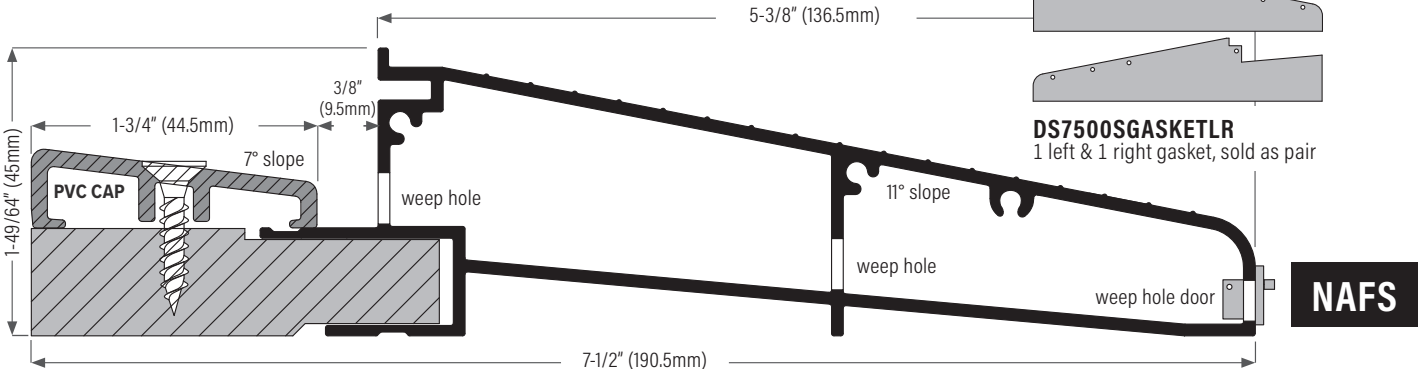
DS7500CVT Clear anodized with pvc tan cap DS7500AVBL Clear anodized with pvc black cap DS7500DVBL Bronze anodized with pvc black cap
