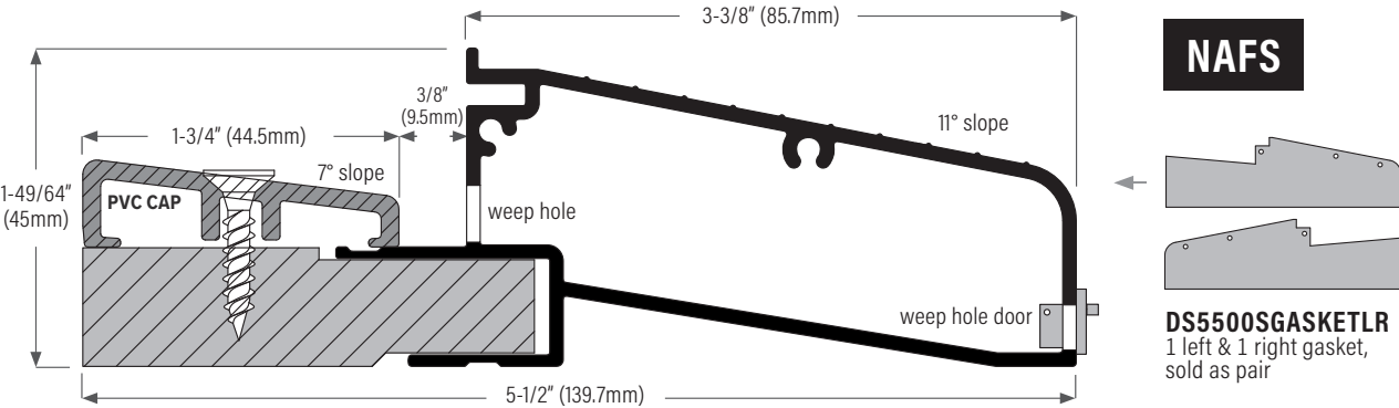
DS5500CVT Clear anodized with pvc tan cap DS5500CVBL Clear anodized with pvc black cap DS5500DVBL Bronze anodized with pvc black cap
