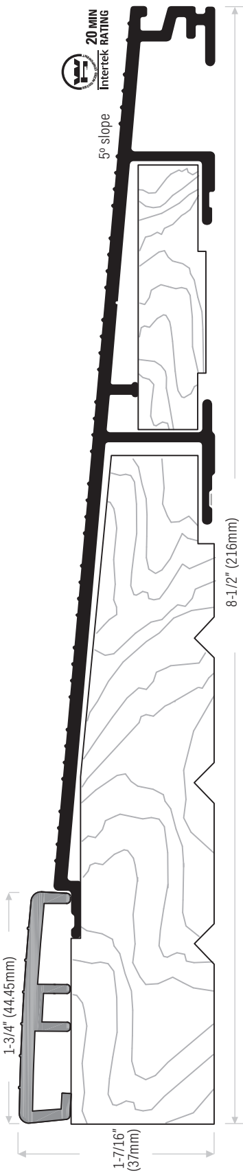
DS814AVT Extruded aluminum sill, mill finish with fixed PVC cap, tan. Length available: 108" (2743mm) only DS814DVBL Bronze anodized with fixed PVC cap, black.
