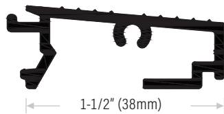
DS1112A150 Extruded aluminum mill finish. Length available: 150" (3810mm) only
