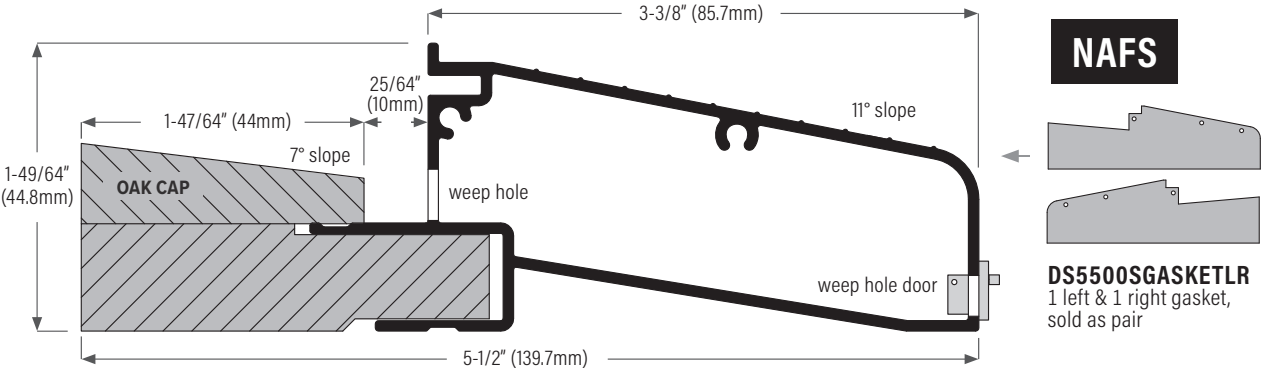
DS5500COAK Clear anodized with oak cap DS5500DOAK Bronze anodized with oak cap
