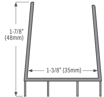
DS129W36 PVC white. 36"
