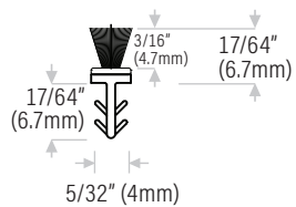
DSP108-20BL 3/16" (4.7mm) pile height, black
