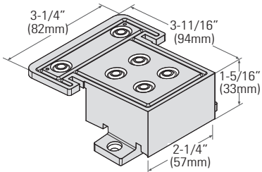
DS725BSPT31116 tan DS725BSPW31116 white DS725BSPBL31116 black For large T-bar 3-11/16" (94mm) depth x 3-1/4" (83mm)
