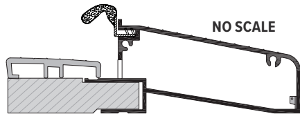
DS421 Used in inswing door sill application
