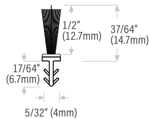
DSP108-50BL 1/2" (12.7mm) pile height, black
